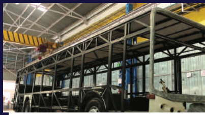
BUS BODY
